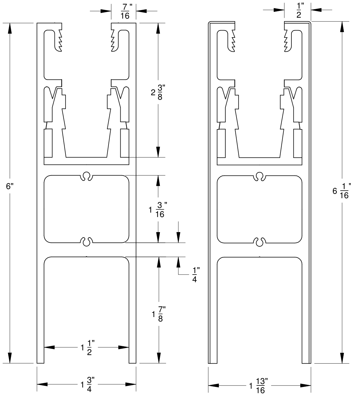
ALUMINUM RAIL
